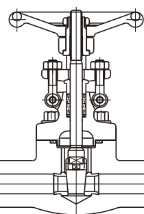
Bolted bonnet OS & Y Hoop connection Solid wedge
