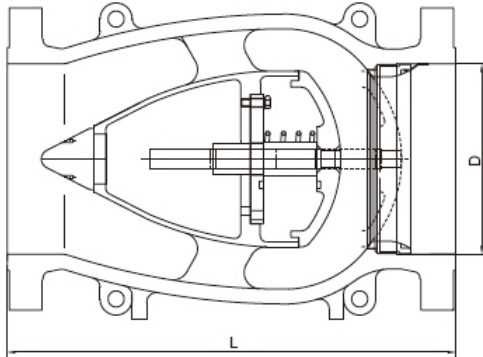
Long pattern
