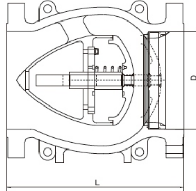
Short pattern
