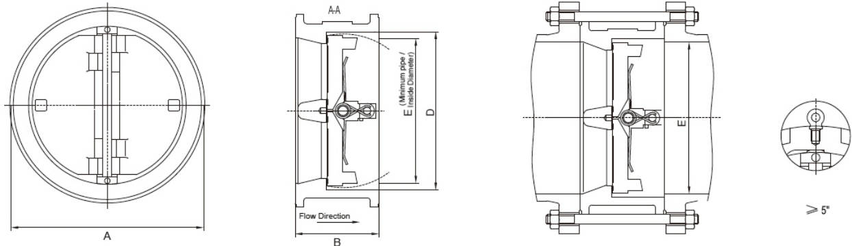
Wafer type
