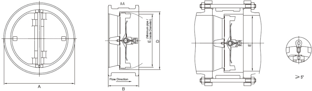
Wafer type
