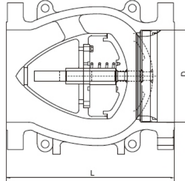
Short pattern
