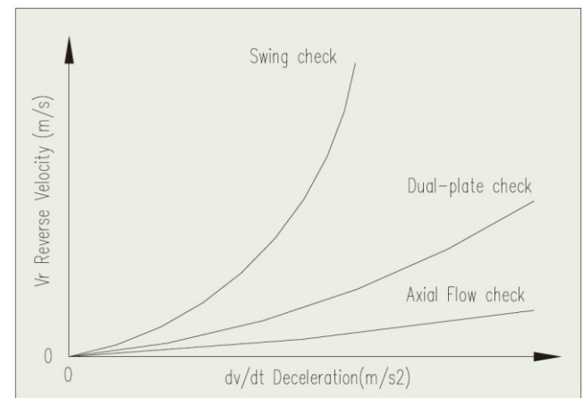
Figure : Dynamic flow performance characteristics.
