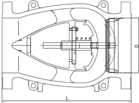
Long pattern
