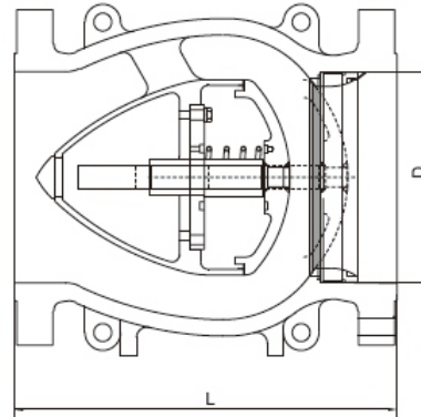
Short pattern
